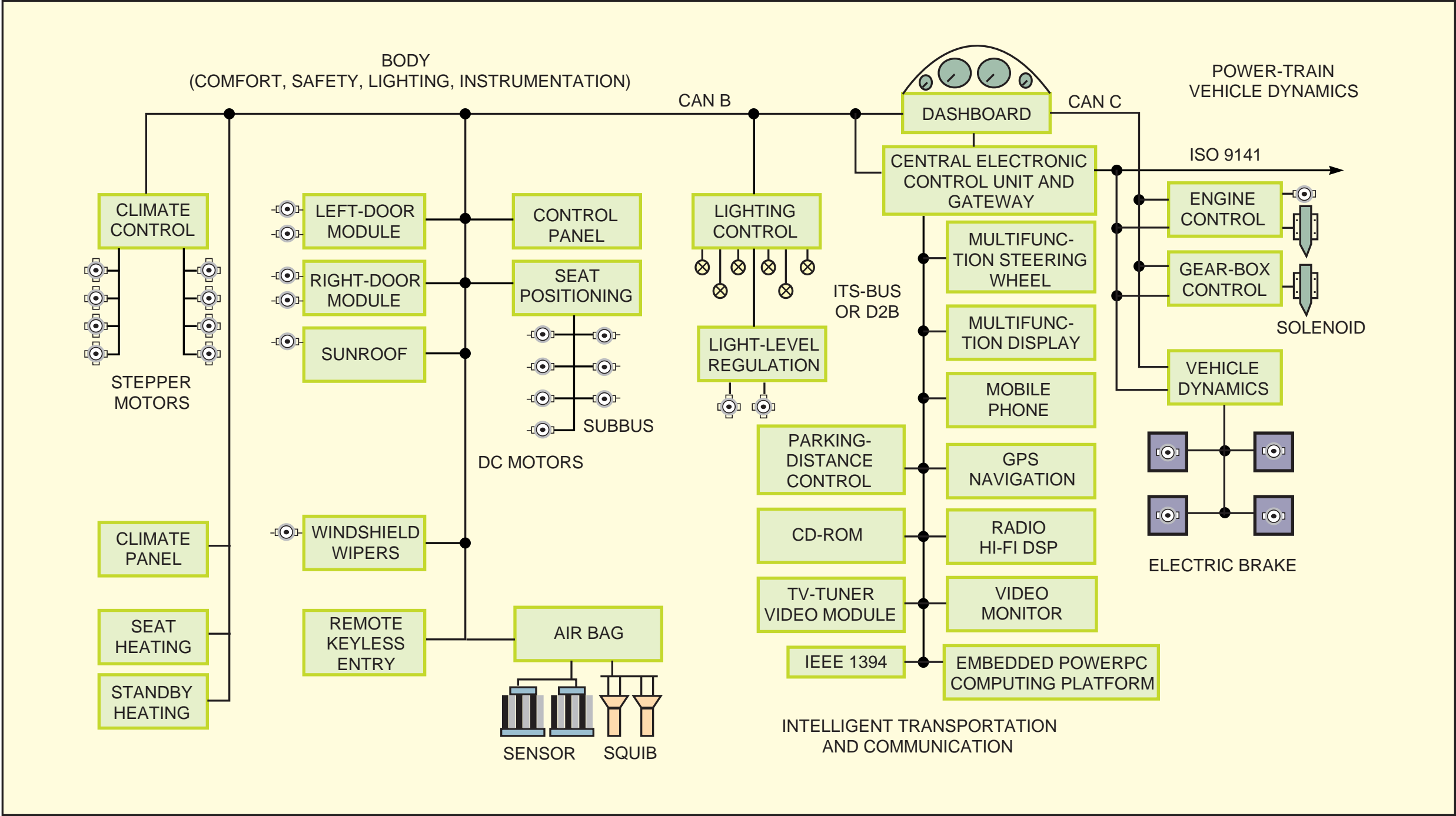
Motorola's version of the SAE's vehicle-network architecture includes a gateway among the CAN C mission-critical functions, the CAN B body functions and the Intelligent Transportation Systems high-speed bus.
