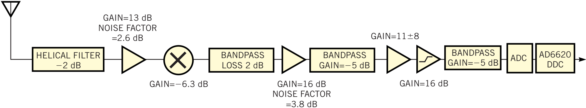
The basic radio comprises a series of stages between the antenna and the ADC, which feeds data to the DSP.
