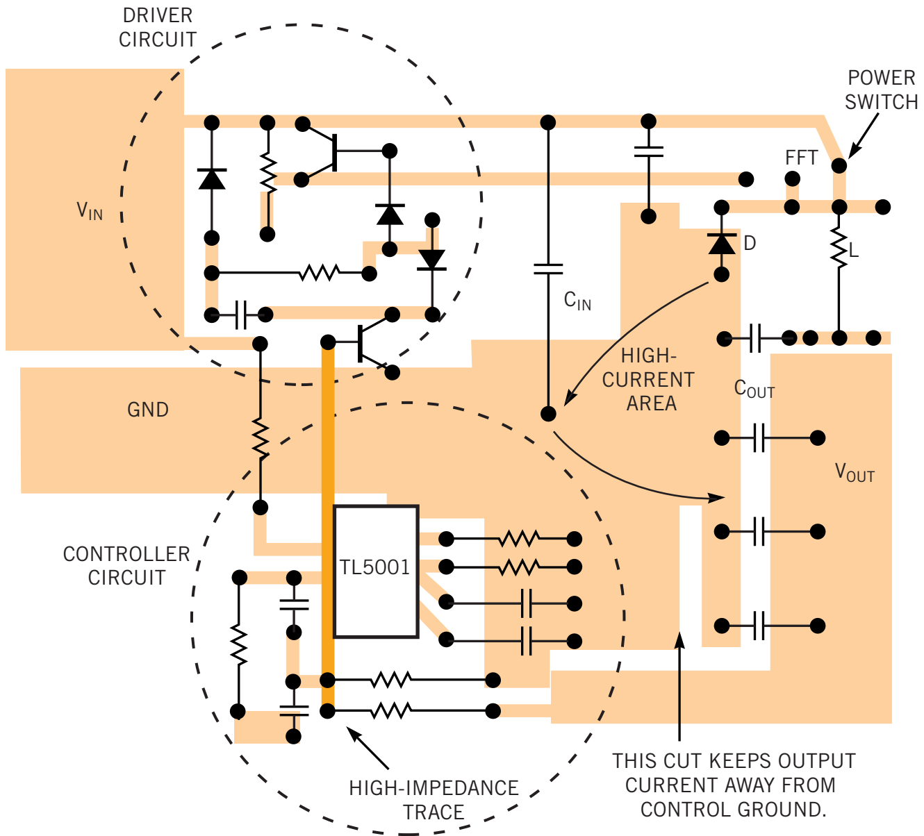
Proper board layout increases power-supply efficiency.
