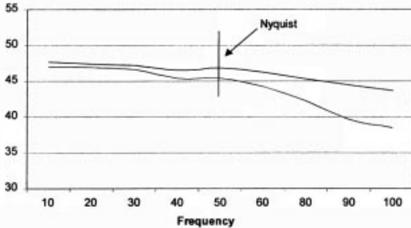
The 8-bit AD9283A/D converter demonstrates high-performance SNR (upper trace) and SINAD (lower trace) for sine-wave inputs of 10 to 100 MHz at its maximum sampling rate of 100M samples/ sec.
