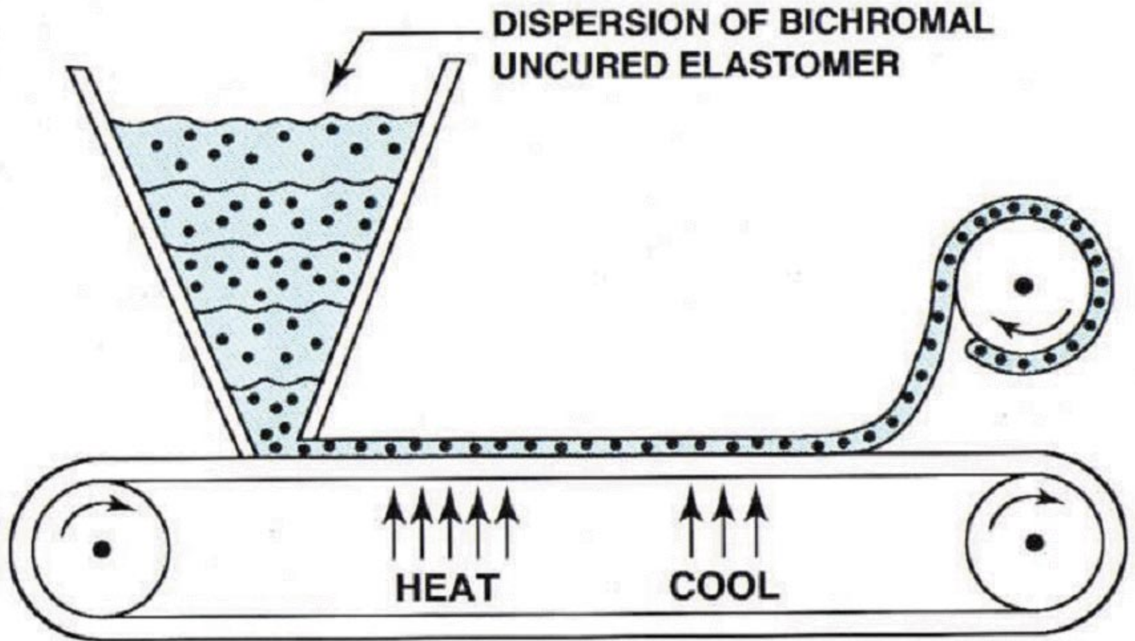
A sheet of electronic paper is produced by curing an extruded mixture of electronic-ink balls and uncured elastomer.
