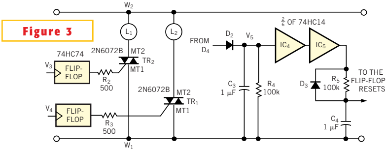
Triacs independently control two loads based on signals from a pair of wall switches.
