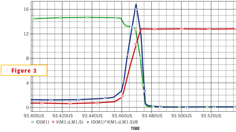
Switching Q_1 results in characteristic waveforms for I_D (green) and V_{DS} (red). The product of these two waveforms gives the instantaneous power dissipation, P_D , (blue).
