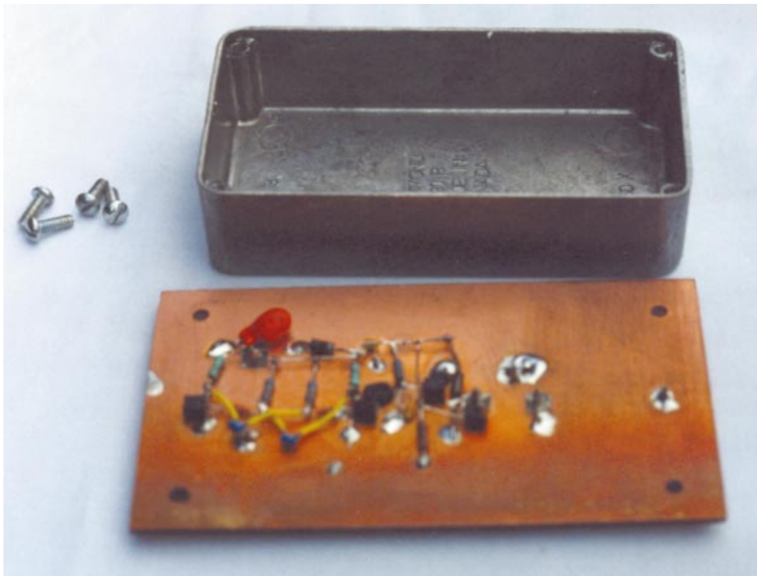
Components all connect to one side of the pc board, and a cast-aluminum cover provides shielding.
