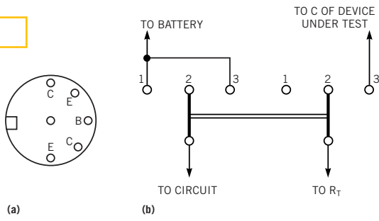
A DIN connector (a) allows you to easily connect transistors; a DPDT switch provides various testing options (b).
