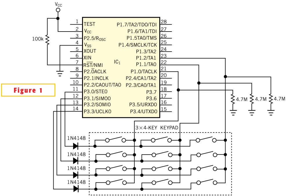
This keypad interface draws only 100 nA in standby mode and avoids “stuck-key” problems.
