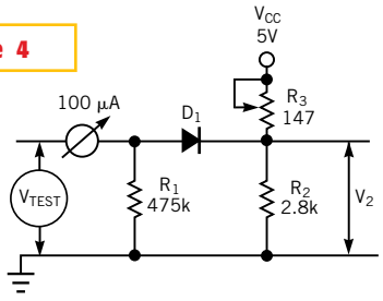
This simple circuit expands the acceptable test results to 90% of full-scale.
