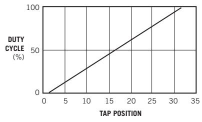
Figure 3 The duty cycle of the Schmitt trigger is a linear function of the potentiometer's tap position.
