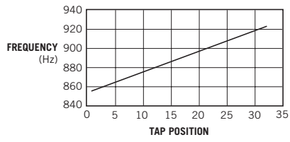
Figure 4 Frequency also varies with the tap position, but with no effect on performance.
