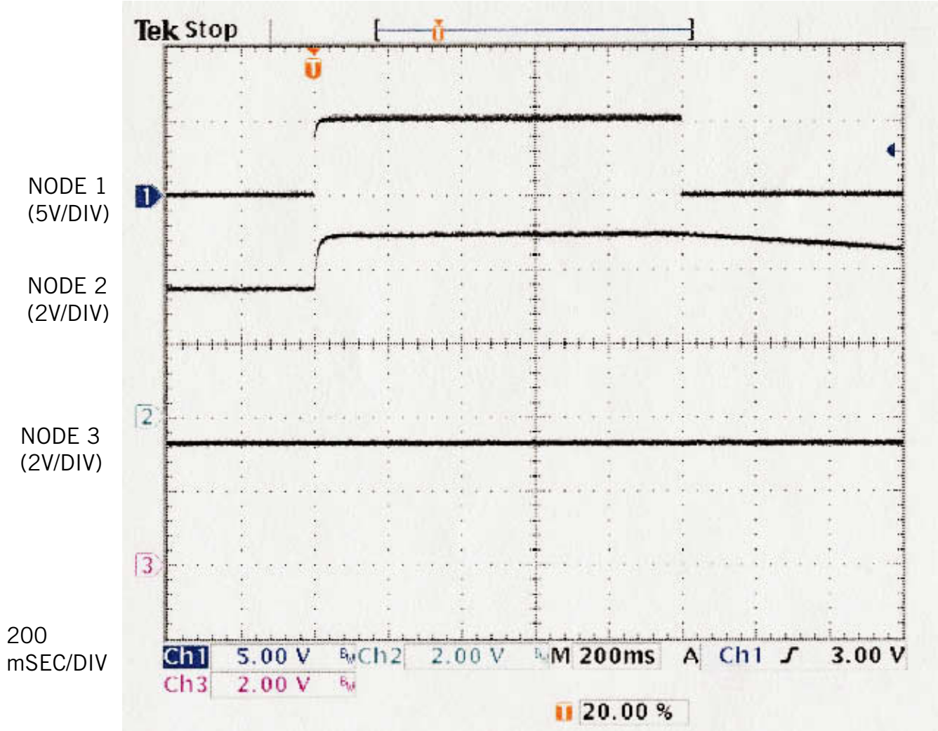
These waveforms (bottom trace, load voltage) show that the load current suffers no interruption during a switchover from USB to battery.
