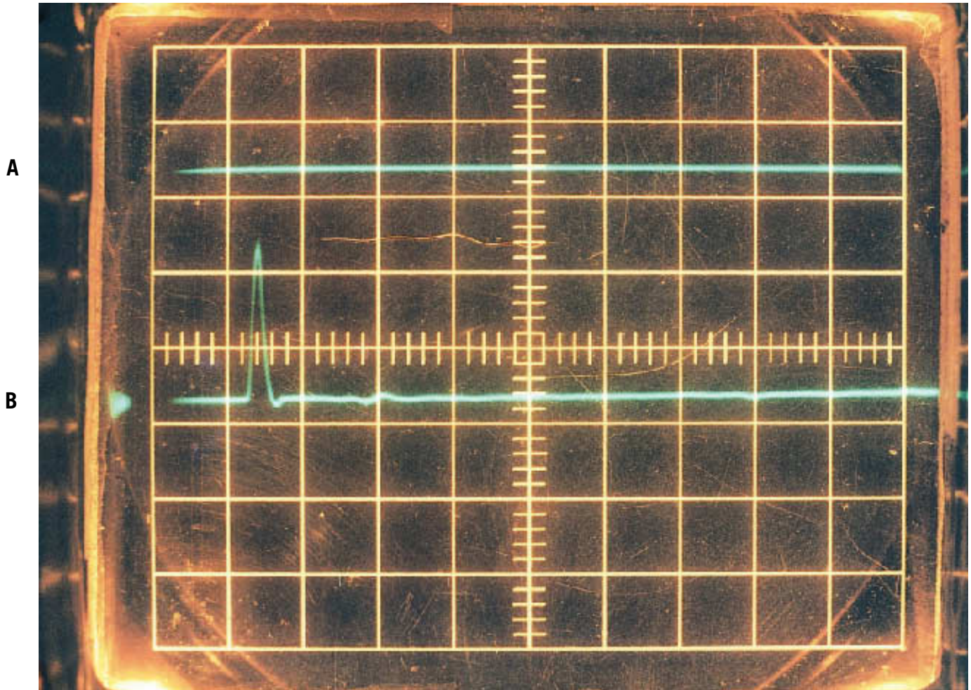
Traces A and B show the impulse response, respectively, without and with the delay network.
