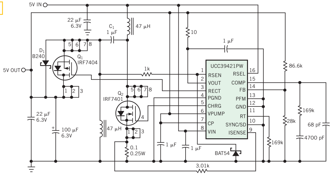
The synchronous SEPIC converter operates over a wide input-voltage range.
