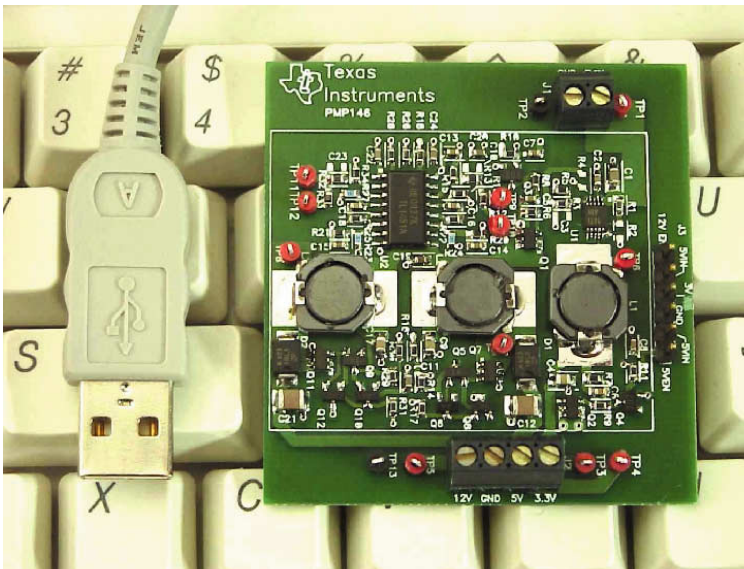
A sample DSL-modem power supply optimized for low cost and efficiency measures only 1.5 \times 3 in.
