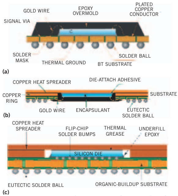
Figure 4 Conventional BGA (a), cavity-down BGA (b) and flip-chip BGA (c) packages deliver different combinations of cost, heat-dissipation, and performance characteristics (courtesy Xilinx).
