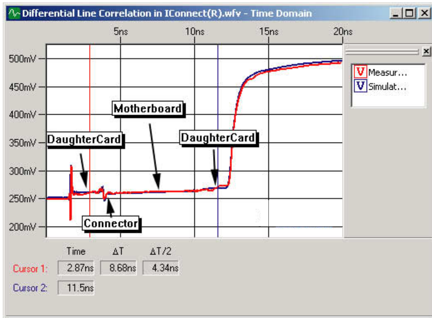
Simulation in Berkeley Spice correlates to TDR measurements for odd mode in a differential backplane assembly.
