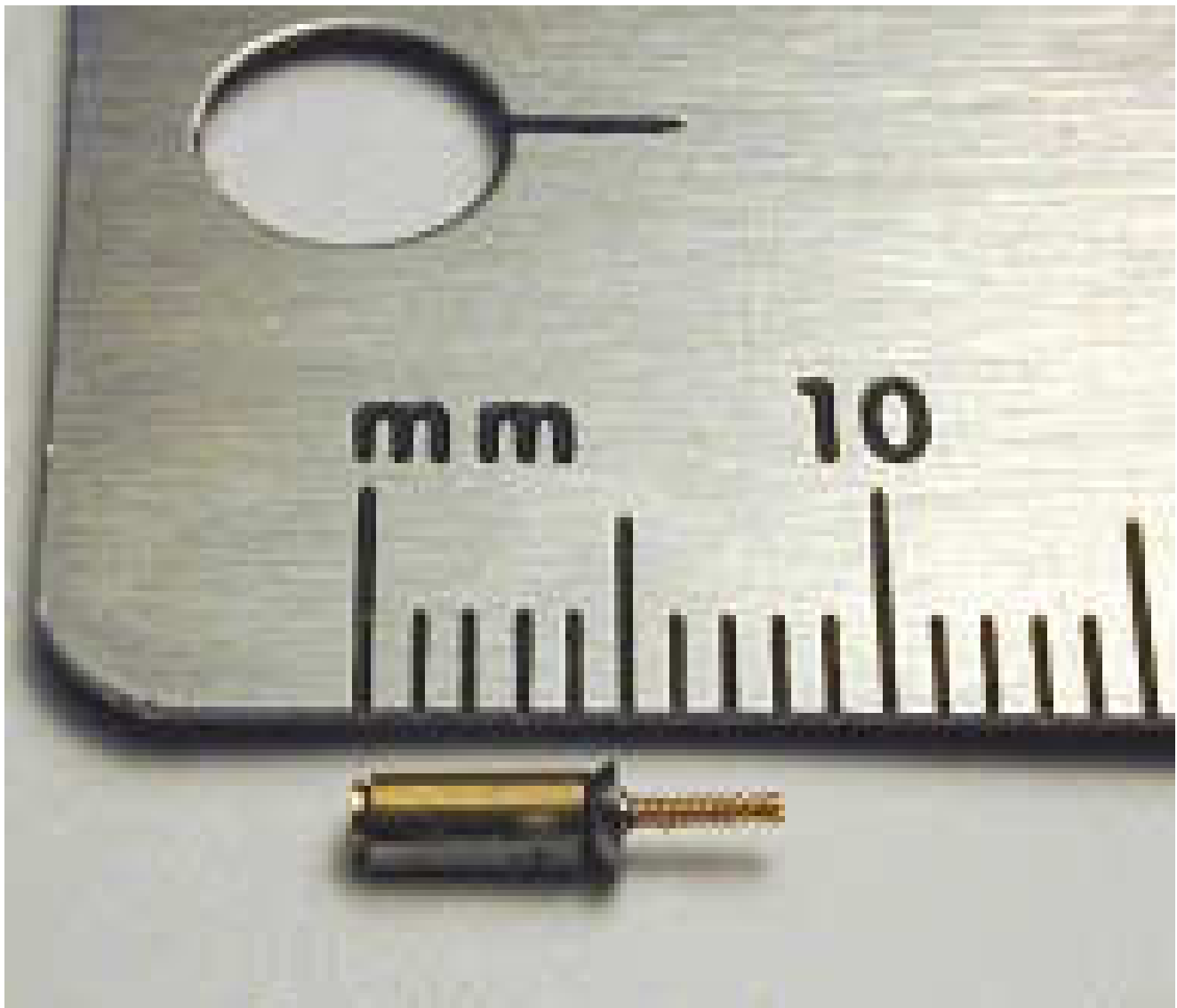
A tiny piezoelectric motor developed at Pennsylvania State University (University Park) produces five times the torque of the smallest electromagnetic motor.
