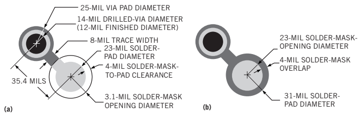
Figure B Compare non-solder-mask-defined pads (a) with solder-mask-defined pads (b), which employ the pc board's solder-resist mask to define the BGA's land areas.
