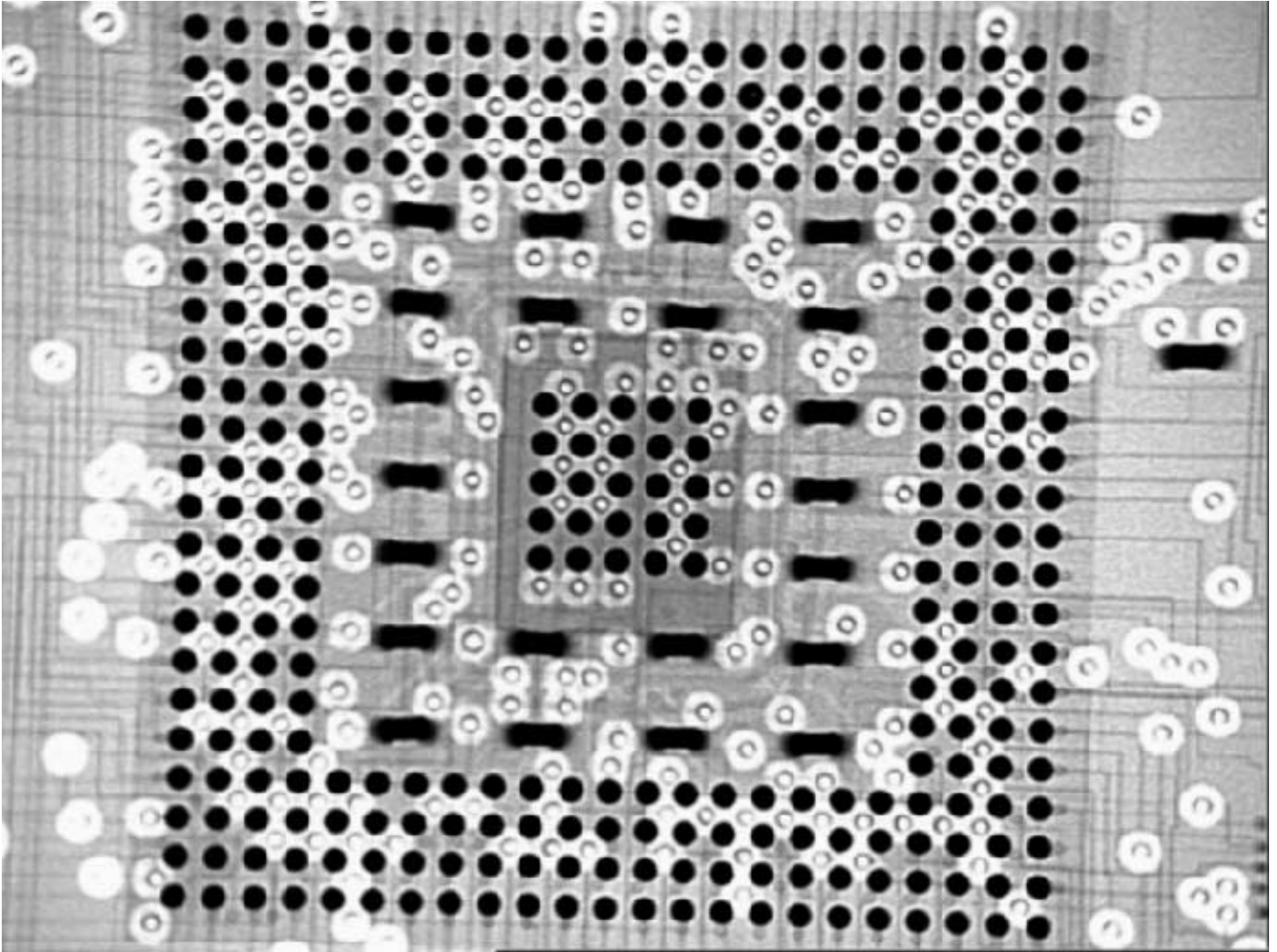
Inspection X-ray photos show that the PBGA perfectly connects with the pc board's SMD pads.
