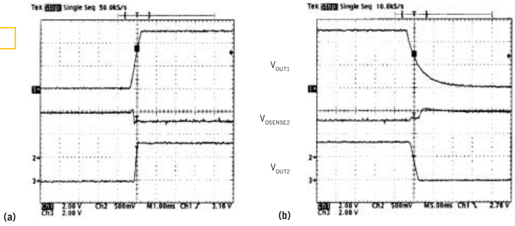
These supply-voltage waveforms occur at turn-on (a) and turn-off (b).
