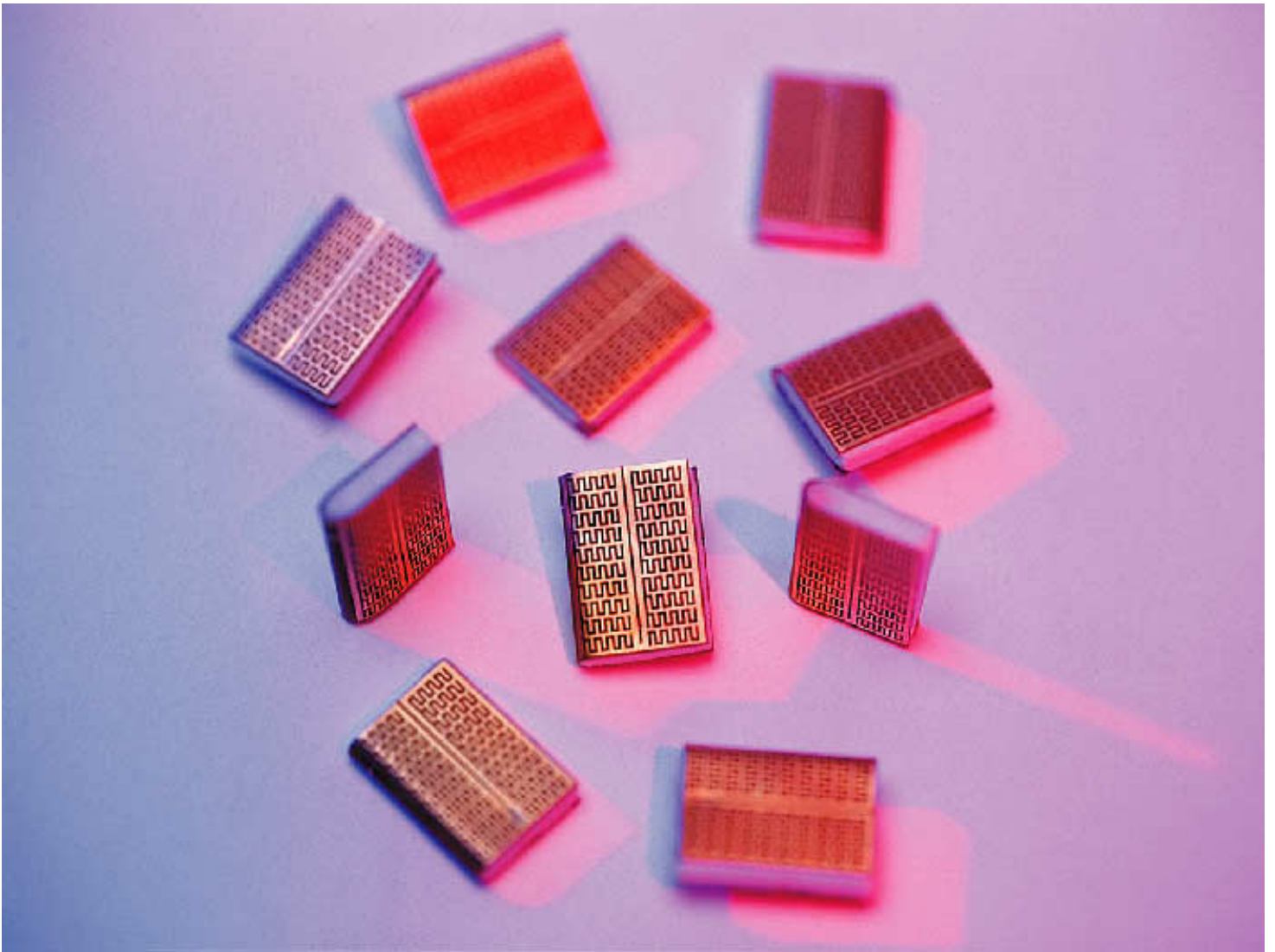
A frequency-selective surface, created by printing patterns of inductors and capacitors on film, is the basis for these 9 \times 13 \times 2.2 -mm ClearLink antennas from e-tenna, which work for 2.4-GHz Bluetooth and 802.11b applications.
