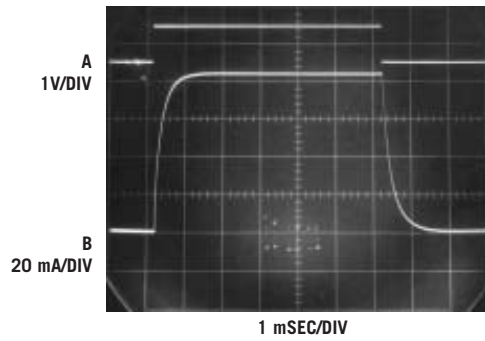
Figure 5 Figure 3's output (Trace B) responds to Trace A's input step. Trace B's laser current has controlled damping and no overshoot.
