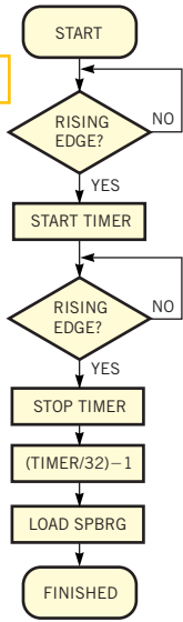
This program-flow diagram illustrates the principles of the baud-rate-detection technique.
