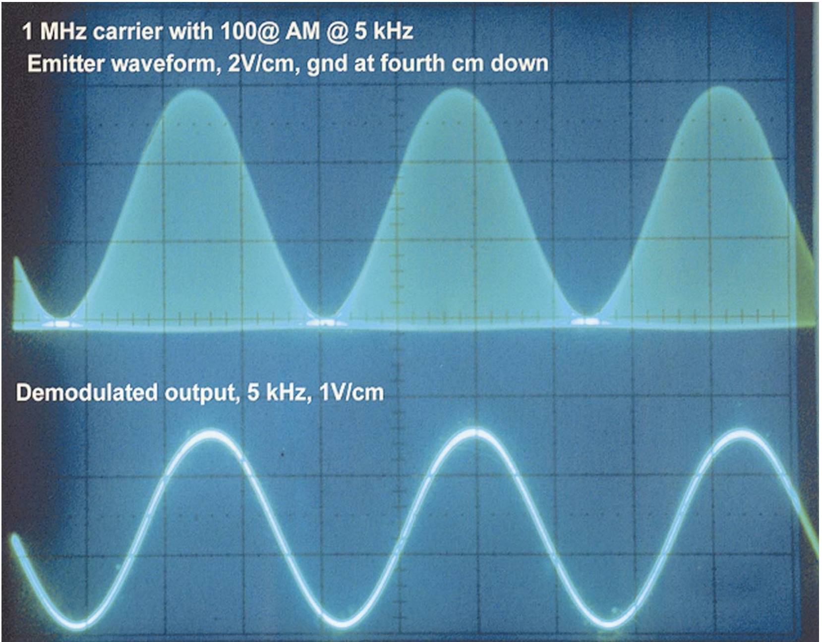
A scope photo shows the running demodulator; the upper trace is the emitter node, and the lower trace is the output.
