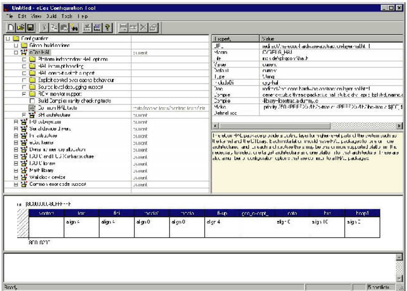
The configuration tool displays a graphical representation of the software packages available in the eCos system.
