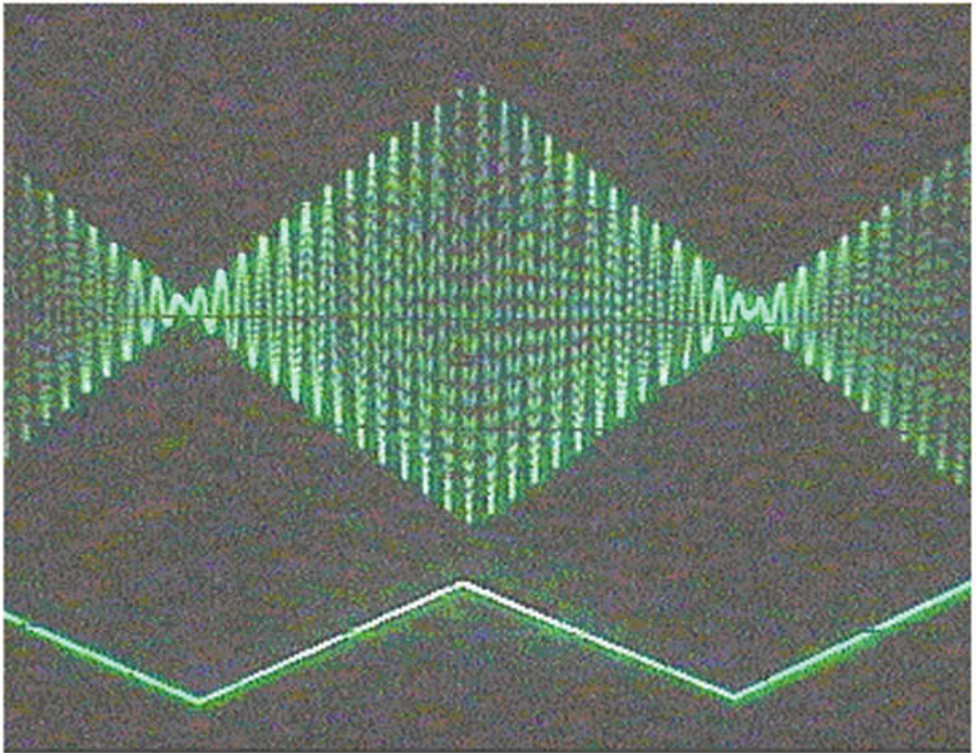
A 0 to 4V triangle wave linearly modulates the 500-Hz audio input.
