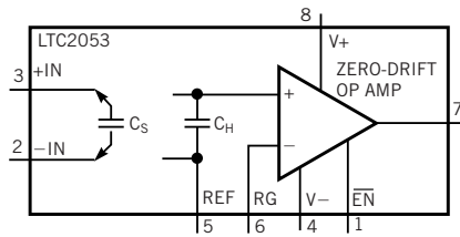
Figure 5 Switched-capacitor techniques can nullify dc errors at the expense of the op amp's becoming another system element that's subject to sampling theory.
