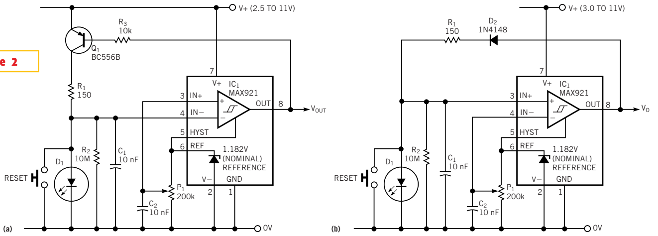
This circuit avoids trip-point changes as a function of supply voltage (a). A modification works from slightly higher supply voltages (b).
