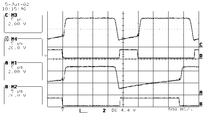
These waveforms typify operation at low (traces C and D) and high (traces A and B) duty cycles.
