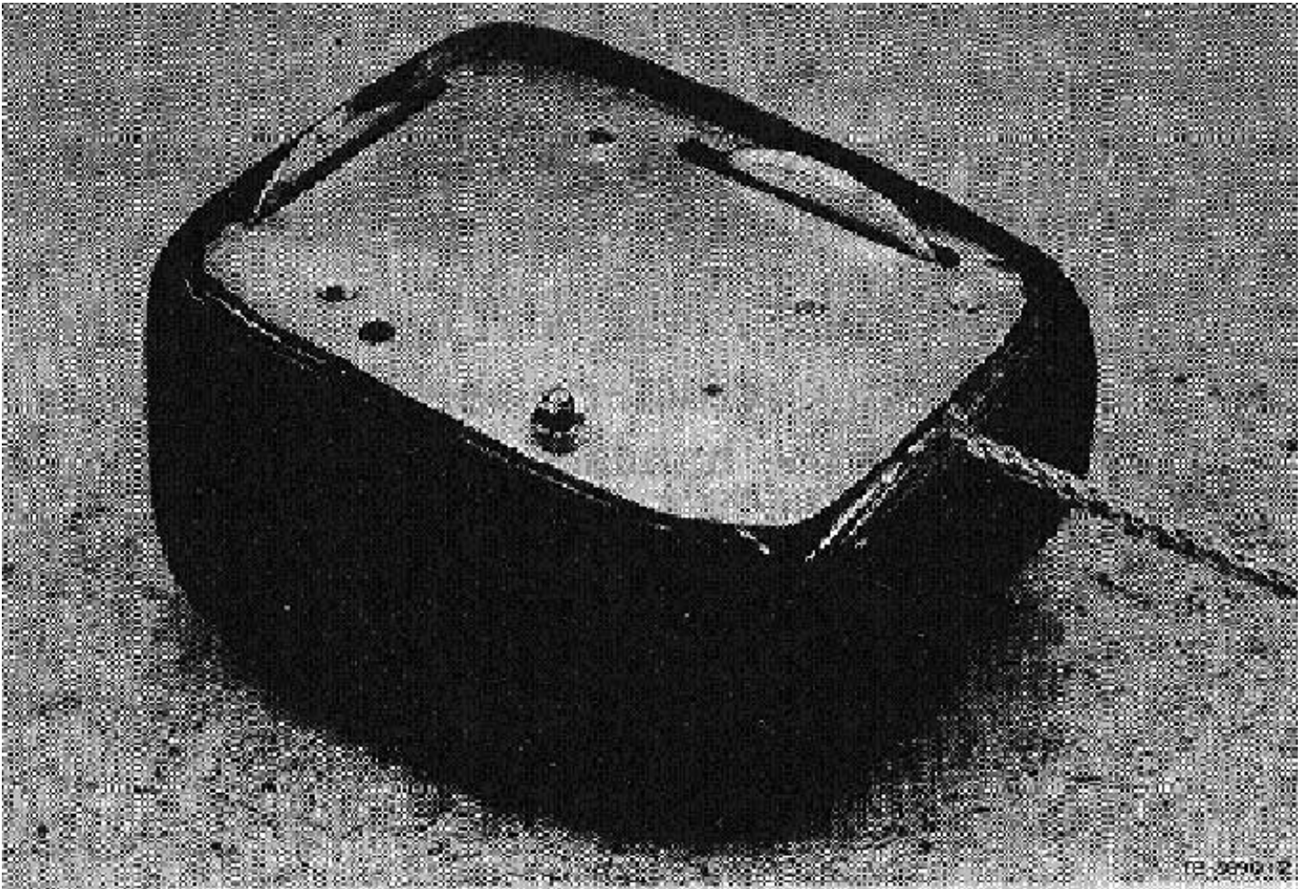
The underside of the mouse prototype shows the two wheels to detect motion. The wheels eventually moved inside the casing, where a ball acts upon them.
