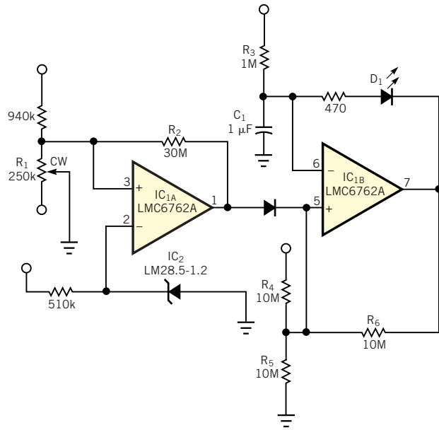
This flepower flasher indicates a low-battery condition with a flashing LED.
