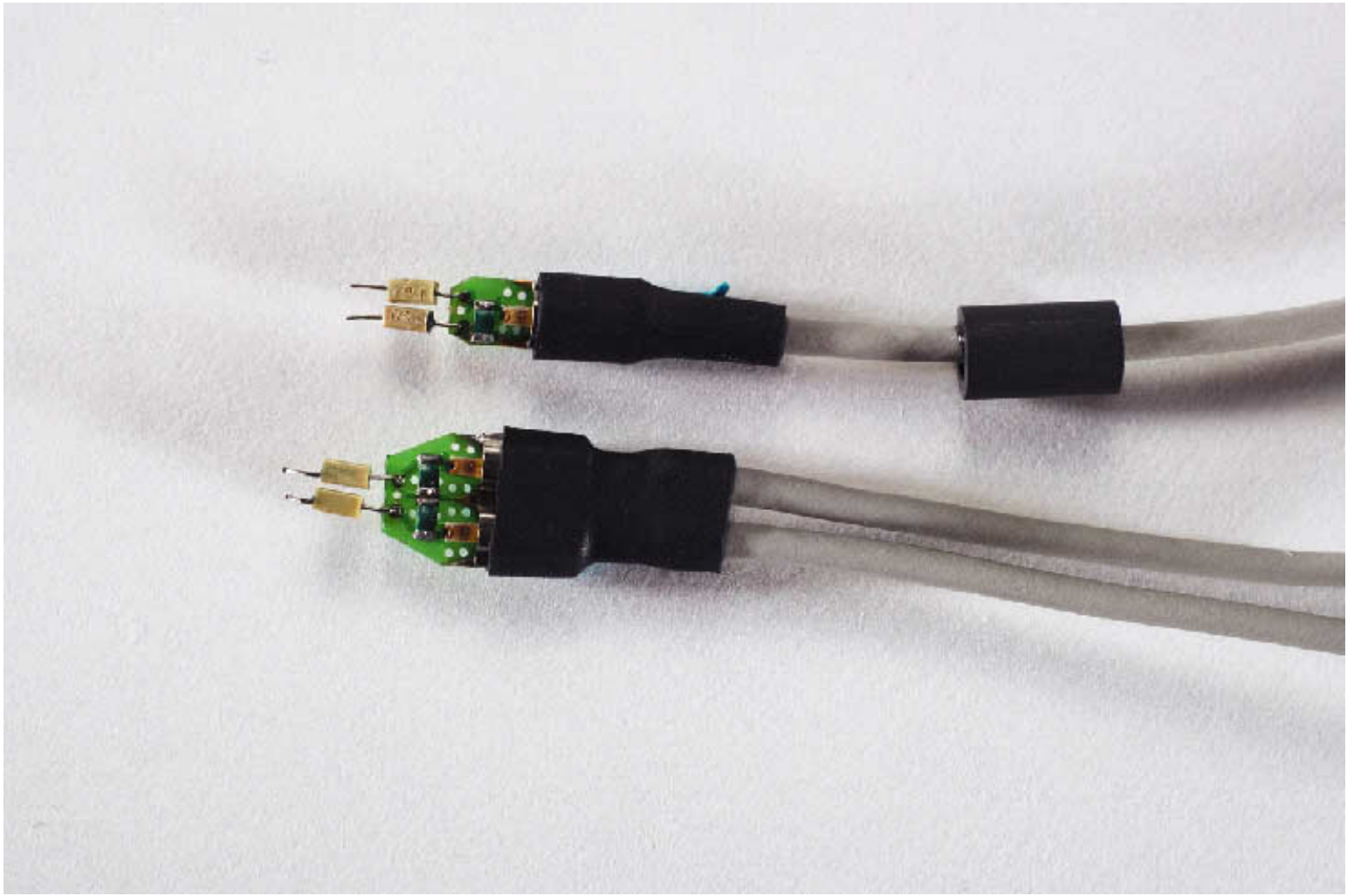
This close-up of single-ended and differential solder-in probe heads shows the single-ended head's greater simplicity and smaller size.
