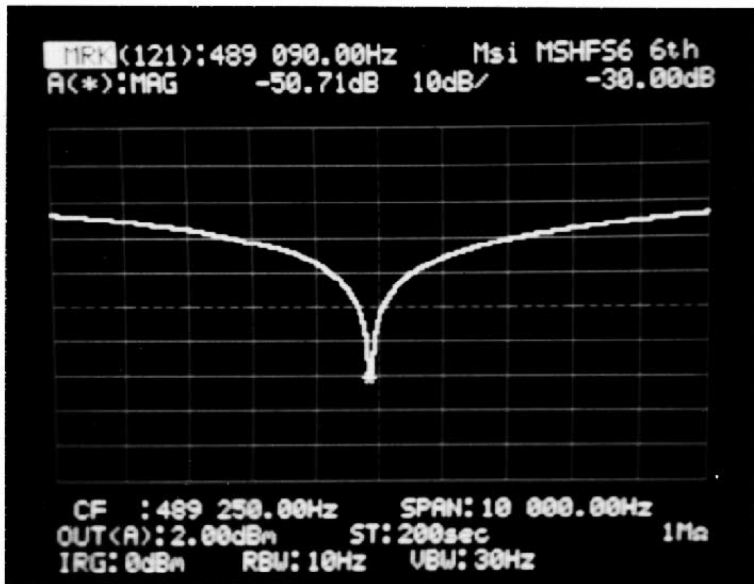
The circuit in Figure 1 delivers a -50-dB notch.
