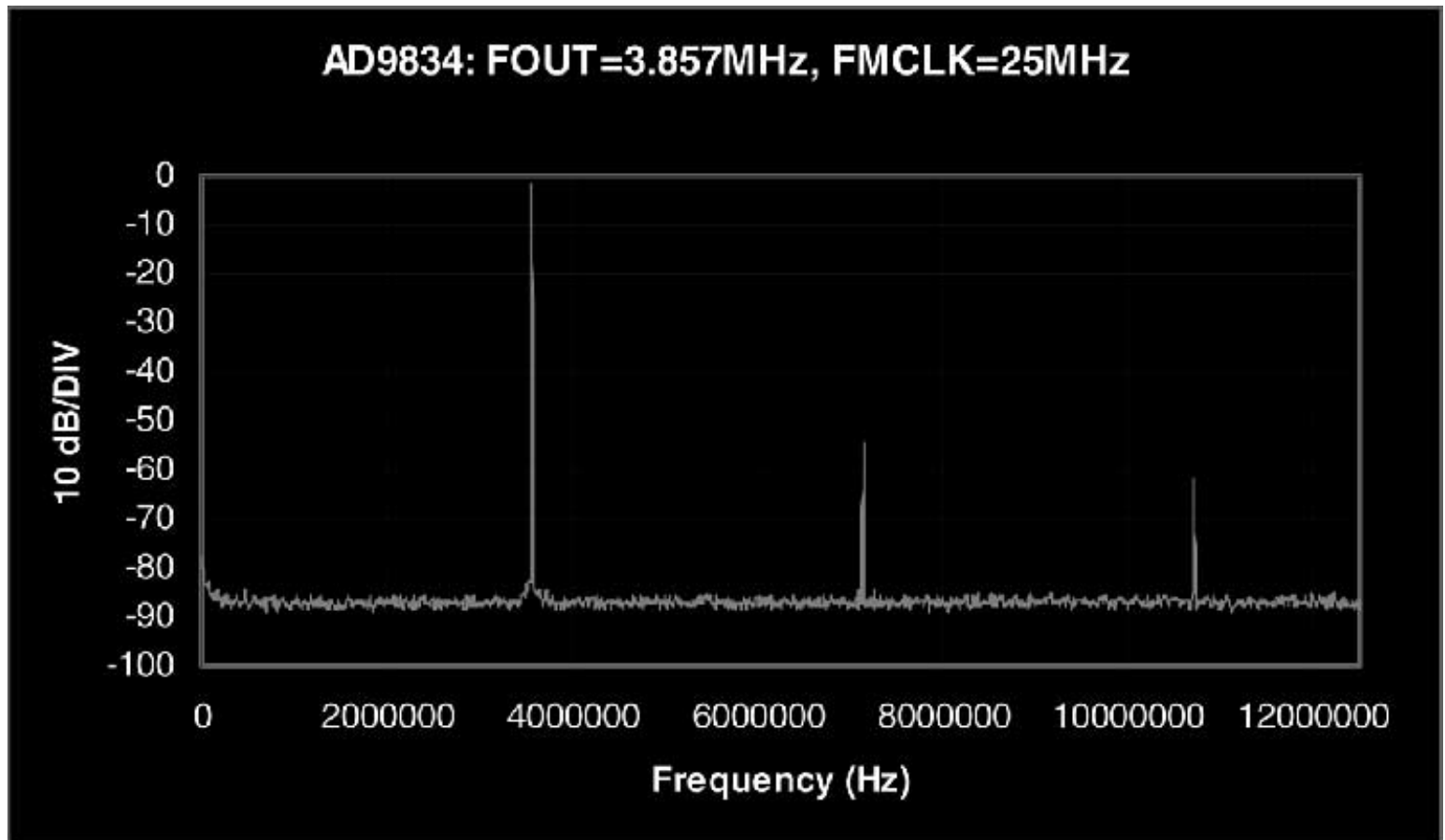
This spectral plot shows the fundamental, second harmonic, and third harmonic for a 3.857-MHz signal.
