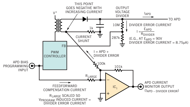
Figure A Feedforward from the programming input compensates for the output voltage divider's current-loading error.
