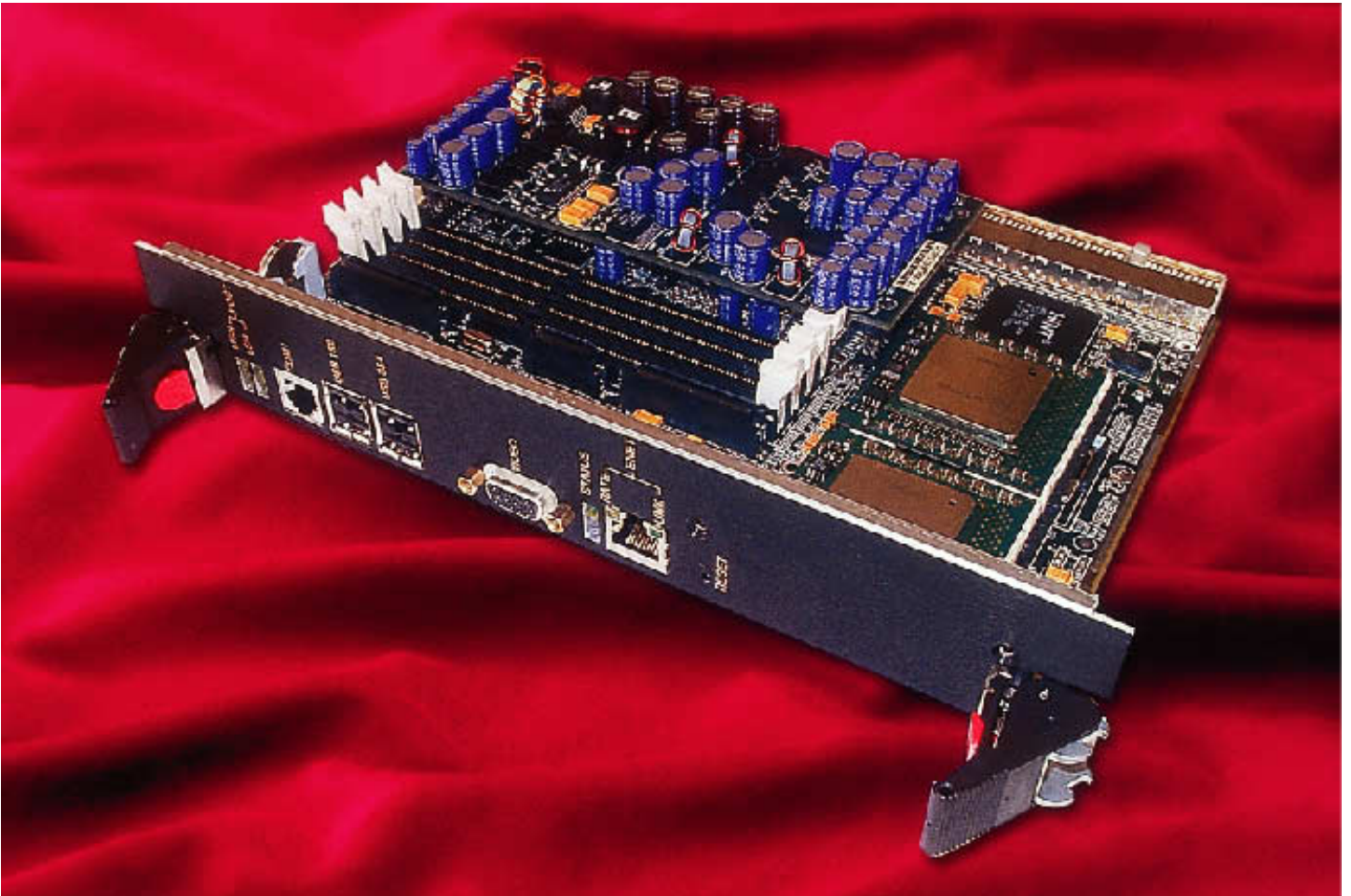
Two low-power Pentium IV Xeon processors with clock speeds approaching 3 GHz power the C269 Equinox single-board computer.
