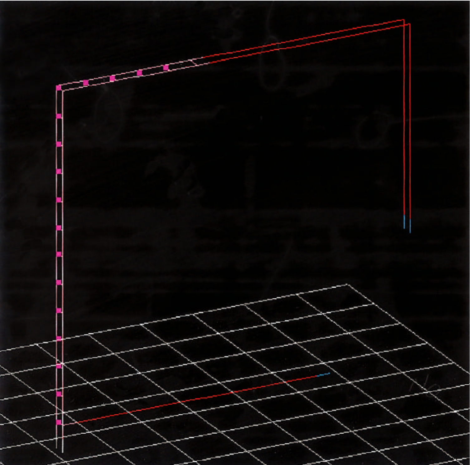
The square grids represent loads of 30\Omega in series with 78-fF capacitors.
