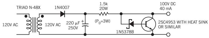
Figure 4 A 100V screen-grid power supply transforms a normal triode into a boosted triode.
