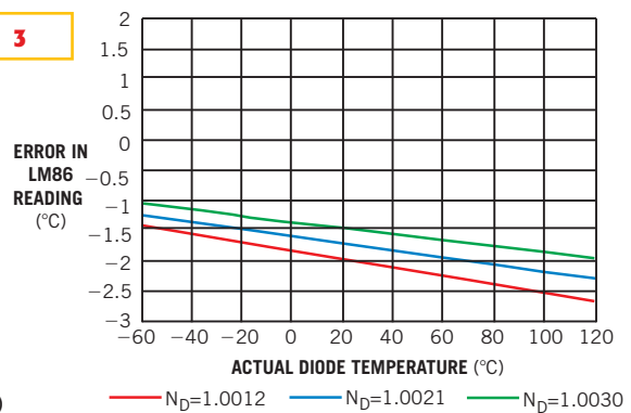
Using the LM86 with a Pentium IV, 0.13-micron CPU results in errors (a). But holding the diode's nonideality factor to tighter tolerances results in much closer minimum and maximum errors (b).
