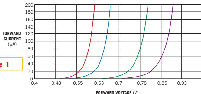
Temperature affects the diode forward voltage.
