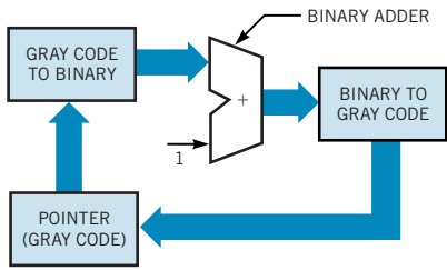
The Gray-code counter, a binary adder, has converters from and to Gray code before and after the adder.
