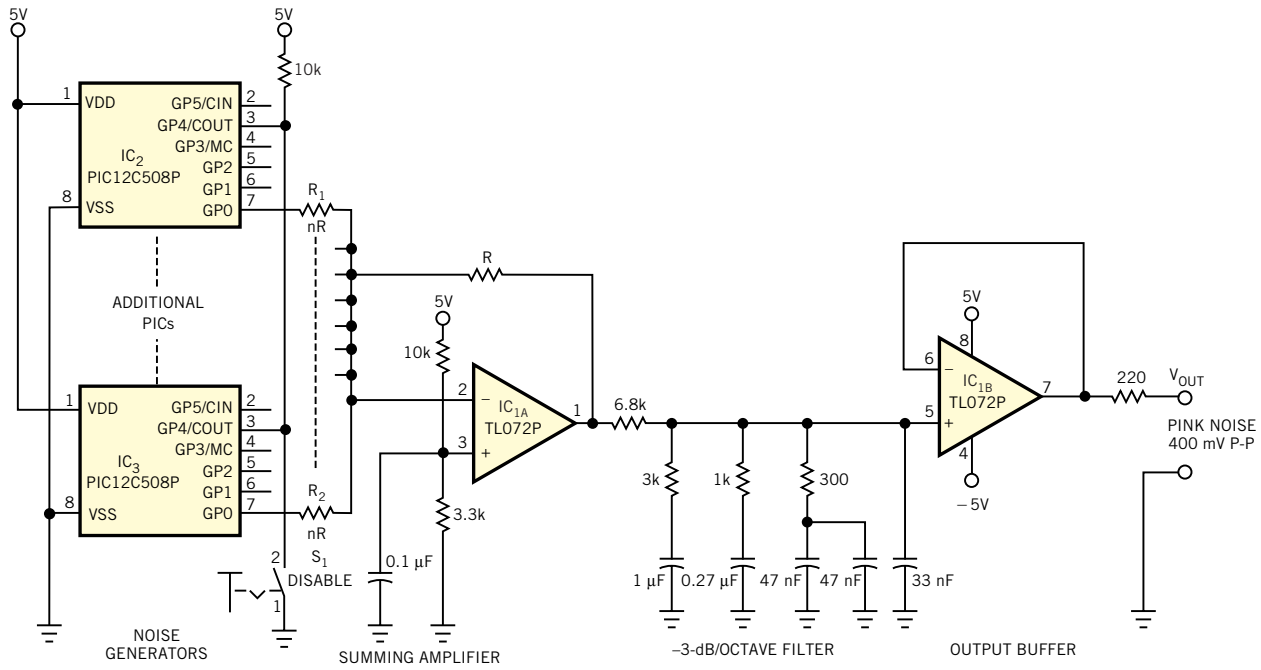
Figure 1 This simple circuit generates Gaussian-distributed noise for audio applications.
