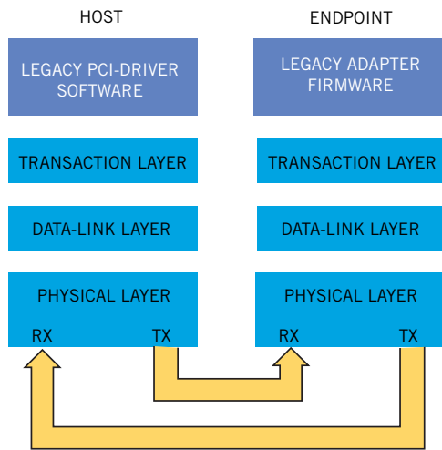
Figure 2 PCI Express has a transaction layer, a data link layer, and a physical layer, although these layers do not represent a physical implementation.
