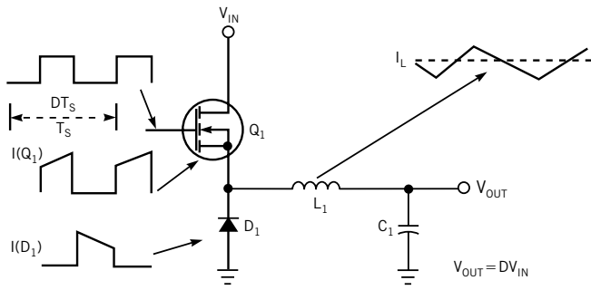
Figure 1 In a typical buck regulator, the output is the switching duty cycle times the input.
