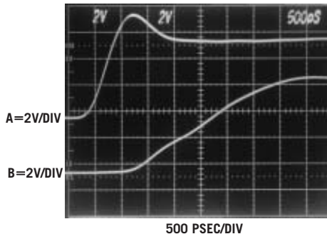
Figure 6 Trace A's 360-psec rise-time pulse completes its transition before the amplifier output (Trace B) begins moving. Trace A's rise time is actually about 150 psec faster than depicted due to the 1-GHz measurement bandwidth that limits the observed response.
