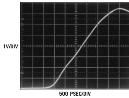
Figure 7 A close examination of the LT1818's response indicates an approximate 2800\text{V}/\mu\text{sec} slew rate, revealing an 11% error in the measurement with a 1-nsec rise-time pulse in Figure 2.
