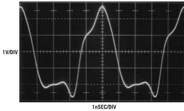
Figure B The time-mark generator output terminated into 50\Omega produces a peaked waveform, which is optimal for verifying timebase calibration.
