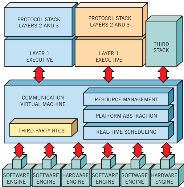
Figure 3 The virtual-machine runtime provides resource management and scheduling, decoupling executives from engines.
